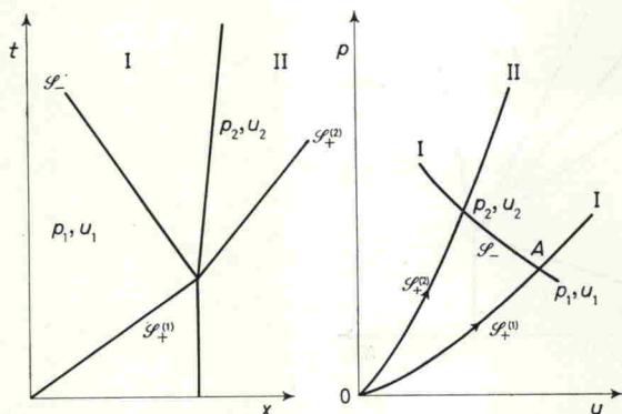
Fig. 10. - Transmission through an interface; \rho_0 D_2 > \rho_0 D_1 .
